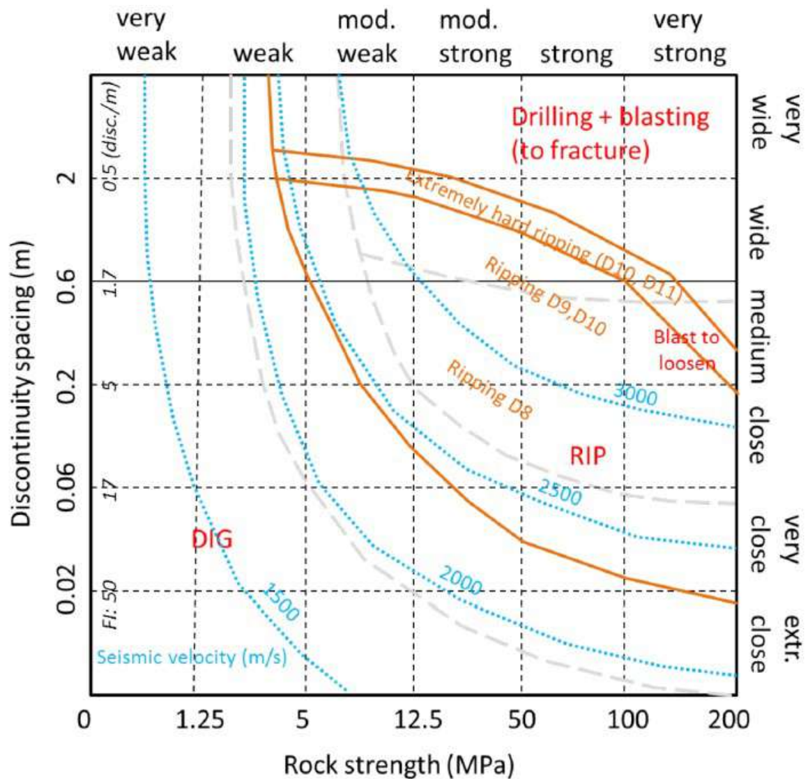
Figure B.3: The boundaries for “Dig”, “Rip” and “Drilling and blasting” for Caterpillar bulldozers given by Pettifer and Fookes (1994), with the fields of the Franklin diagram in the background. In the “Extremely hard ripping” area, excavation is often assisted by hydraulic hammering.
