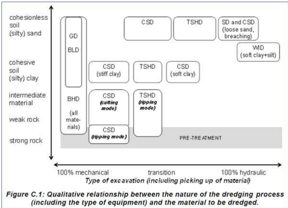
Figure 7.1 Guidance on Application of the Classification: Excavation
