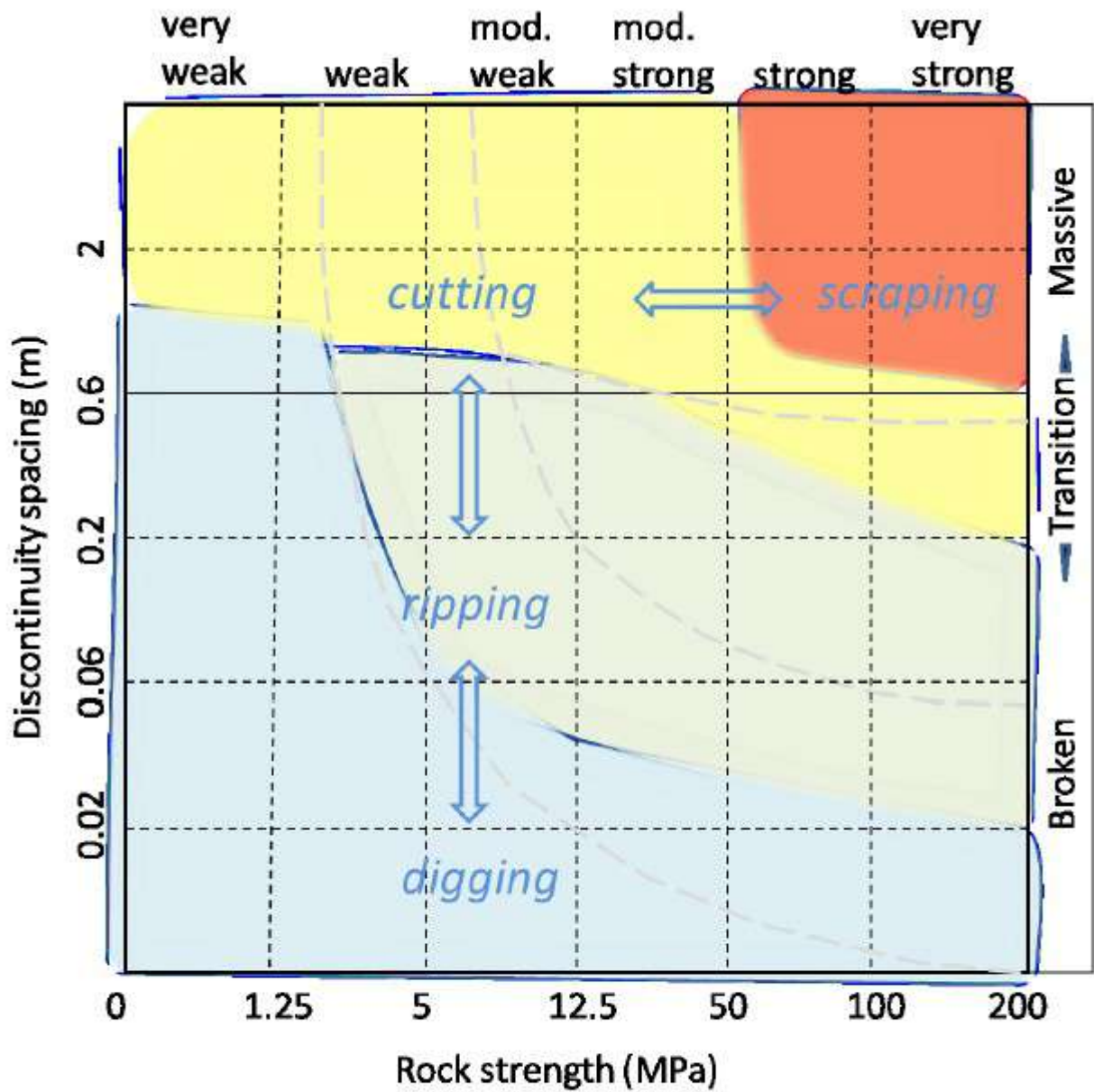
Figure B.4: Rock excavation mechanism fields plotted on excavatability chart. The coloured fields for digging, ripping, cutting and scraping are machine dependent, and will be unique for each type of rock cutting dredger
